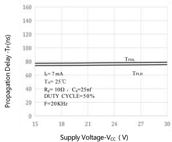
Fig.8 Propagation Delay vs Supply Voltage
