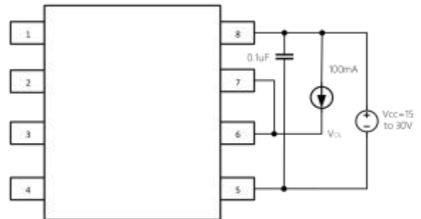
Figure.15 V_{OL} Pulsed Test Circuit
